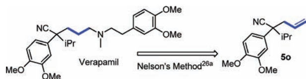
Scheme 5. Verapamil Intermediate
